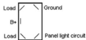
DS-1814 Toggle Switch
