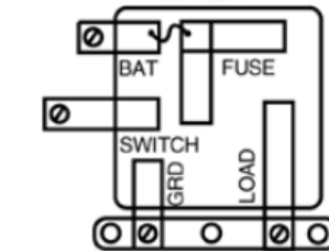
LR-32 Multi-Function Relay 1116969; 6D6306 Cadillac..... 1967 - 1965
