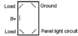
DS-1816 Toggle Switch
