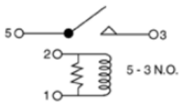
RY-209 A/C Control Relay 39794SE0004; 39794SE0004; RC2203
