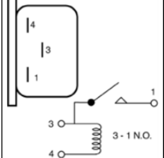
HR-118 Horn Relay
