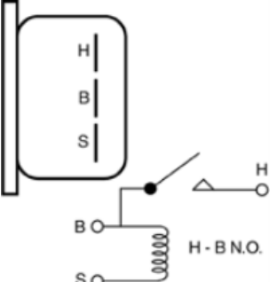
HR-106 Horn Relay
