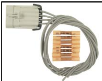
S-1642 Body Harness Connector 12102490
