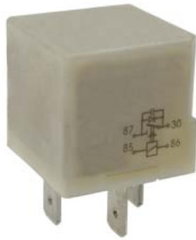
RY-1709 A/C Auto Temperature Control Relay 443919578C
