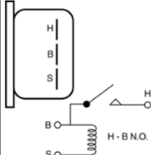
HR-114 Horn Relay
