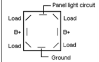
DS-1818 Toggle Switch
