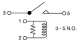
RY-211 A/C Condenser Fan Motor Relay 39795SB2003; 39795SK7003; RC2221
