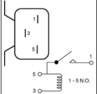
HR-119 Horn Relay
