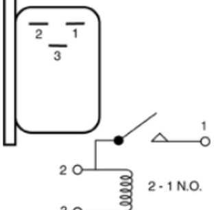
HR-117 Horn Relay
