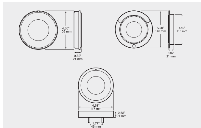
2219F-C features two mounting studs on rear
