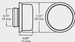
B186-10 bracket (bracket and light sold separately)
