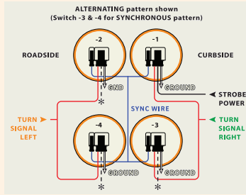
TRADITIONAL 36 DIODE PIRANHA®
