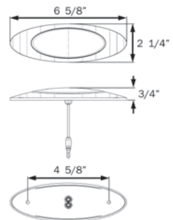
HOLE CUT-OUT: 1.5"
