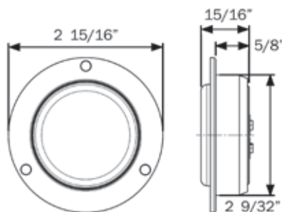
HOLE CUT-OUT: 2.313"
