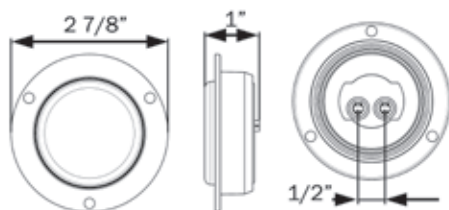
HOLE CUT-OUT: 2.313"
