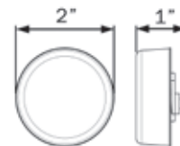
HOLE CUT-OUT: 2.313"
