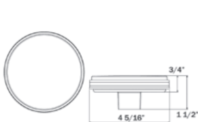
HOLE CUT-OUT: 4.5"
