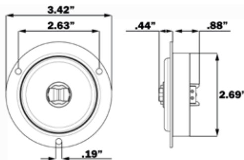
HOLE CUT-OUT: 2.75"
