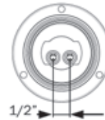
HOLE CUT-OUT: 2.313"
