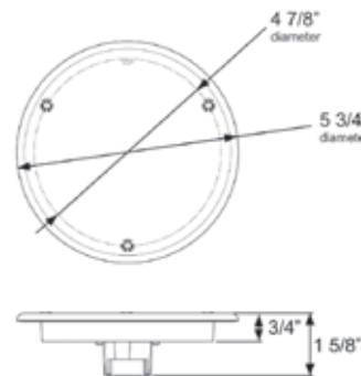
HOLE CUT-OUT: 4.5"
