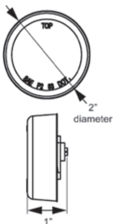
HOLE CUT-OUT: 2.313"
