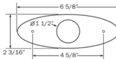
HOLE CUT-OUT: 1.5"
