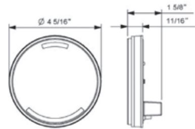
HOLE CUT-OUT: 4.5"
