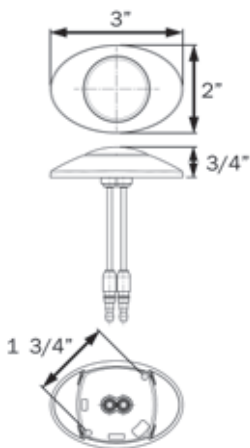
HOLE CUT-OUT: 1.375"
