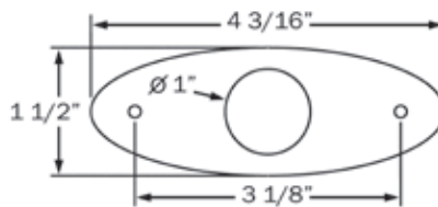
HOLE CUT-OUT: 1"
