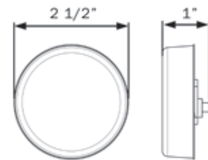
HOLE CUT-OUT: 2.75"
