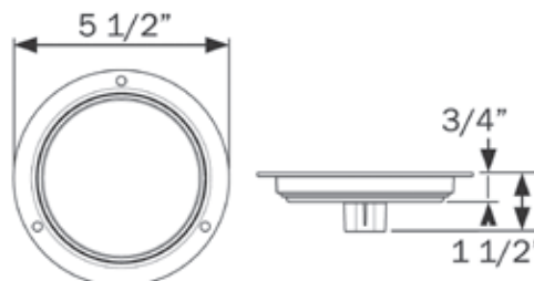
HOLE CUT-OUT: 4.5"
