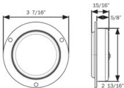
HOLE CUT-OUT: 2.75"
