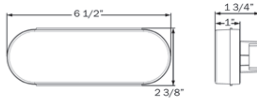
HOLE CUT-OUT: 6.85" x 2.52" (1.26" R)
