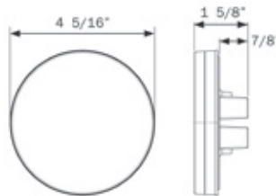
HOLE CUT-OUT: 4.5"
