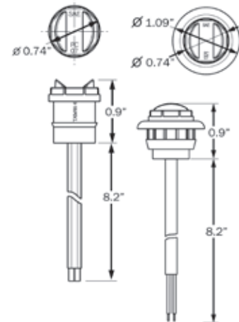
HOLE CUT-OUT: 0.75"
