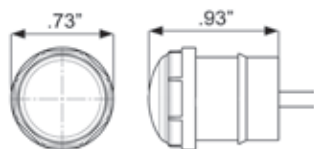
HOLE CUT-OUT: .75"
