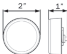
HOLE CUT-OUT: 2.313"
