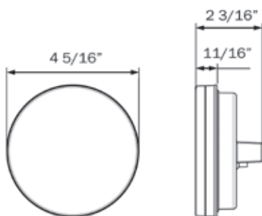
HOLE CUT-OUT: 4.5"
