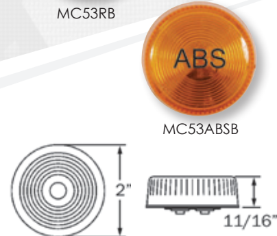
HOLE CUT-OUT: 2.313"
