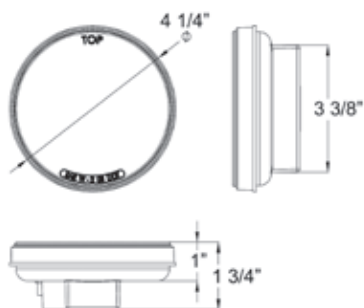
HOLE CUT-OUT: 4.5"
