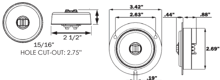
weathertight connection: MCL58AMFB/RMFB
