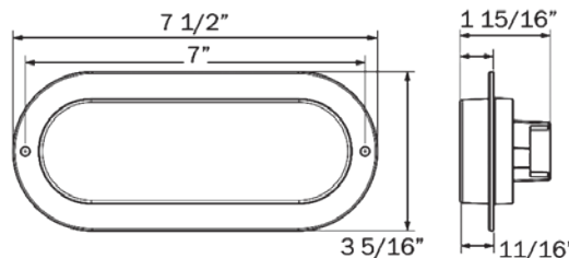
HOLE CUT-OUT: 6.85" X 2.5" (1.25" R)
